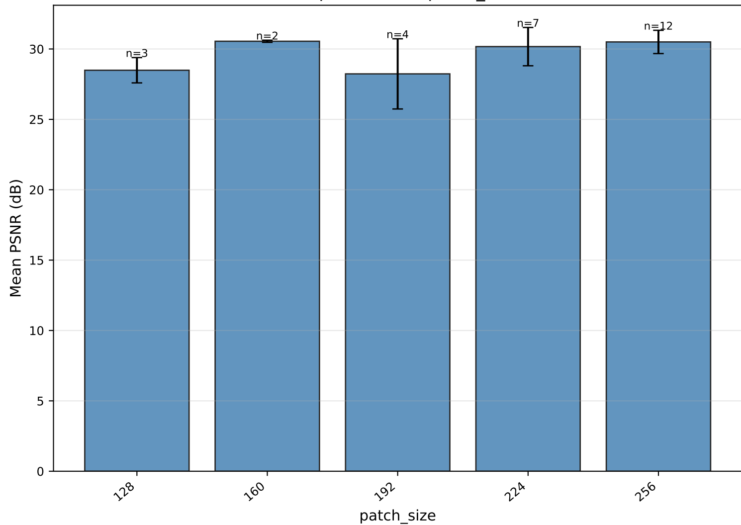
Mean PSNR per value of patch_size — HAT
